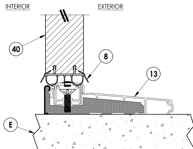
1 VERTICAL CROSS SECTION 8 Inswing Threshold
