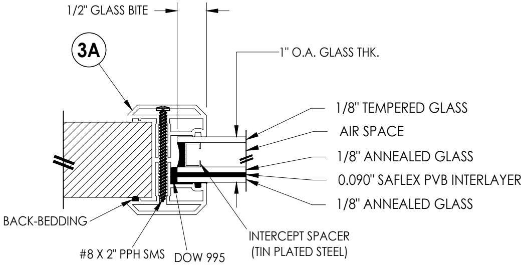
G1 GLAZING DETAIL ODL LITE FRAME ALUMINUM
